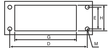
Panel Cutout
