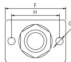
For TNOC-12/16
