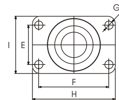
For TNOC-22/28/36/48
